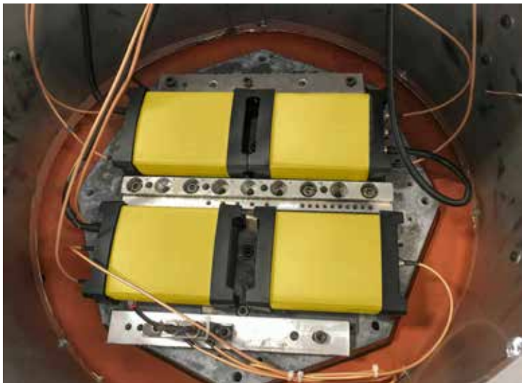
| Vibration Test with Superimposed Temperature Cycle ISO 16750-3
