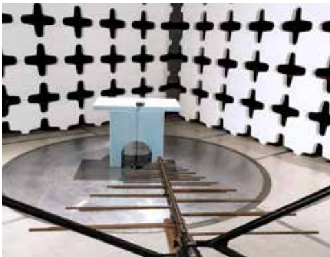
| Ferrite-lined Shielded Test Chamber
